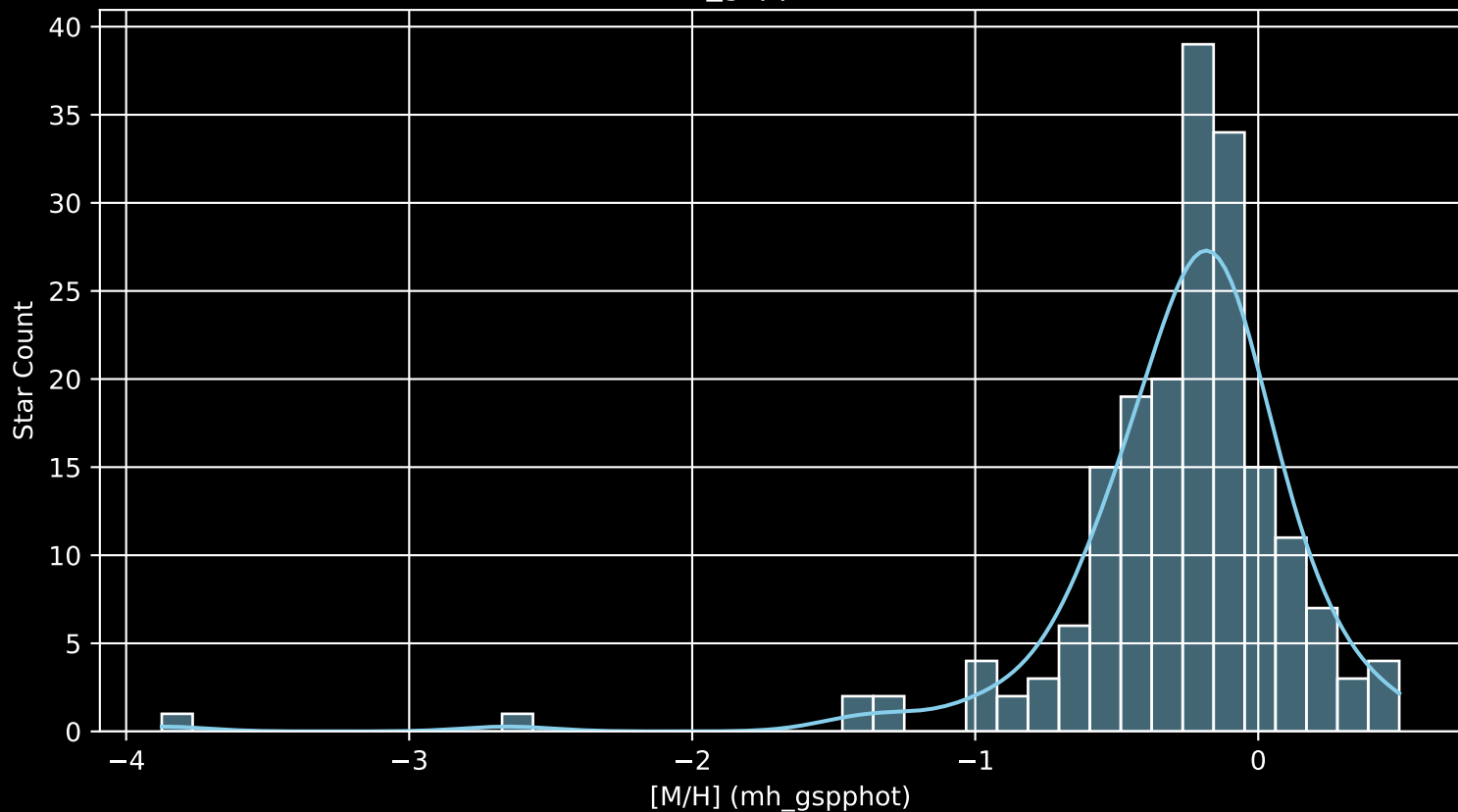
APOGEE DR17 Field: [K2_C6_321+50_btx [M/H] (mh_gspphot) (n= 188)
