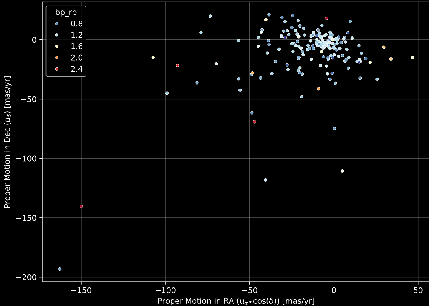
APOGEE DR17 Field: [K2_C6_321+50_btx] Proper Motion Diagram (n= 189)
