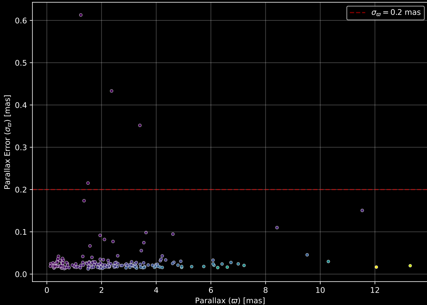
APOGEE DR17 Field: [K2_C6_321+50_btx] Parallax Quality (n= 189)
