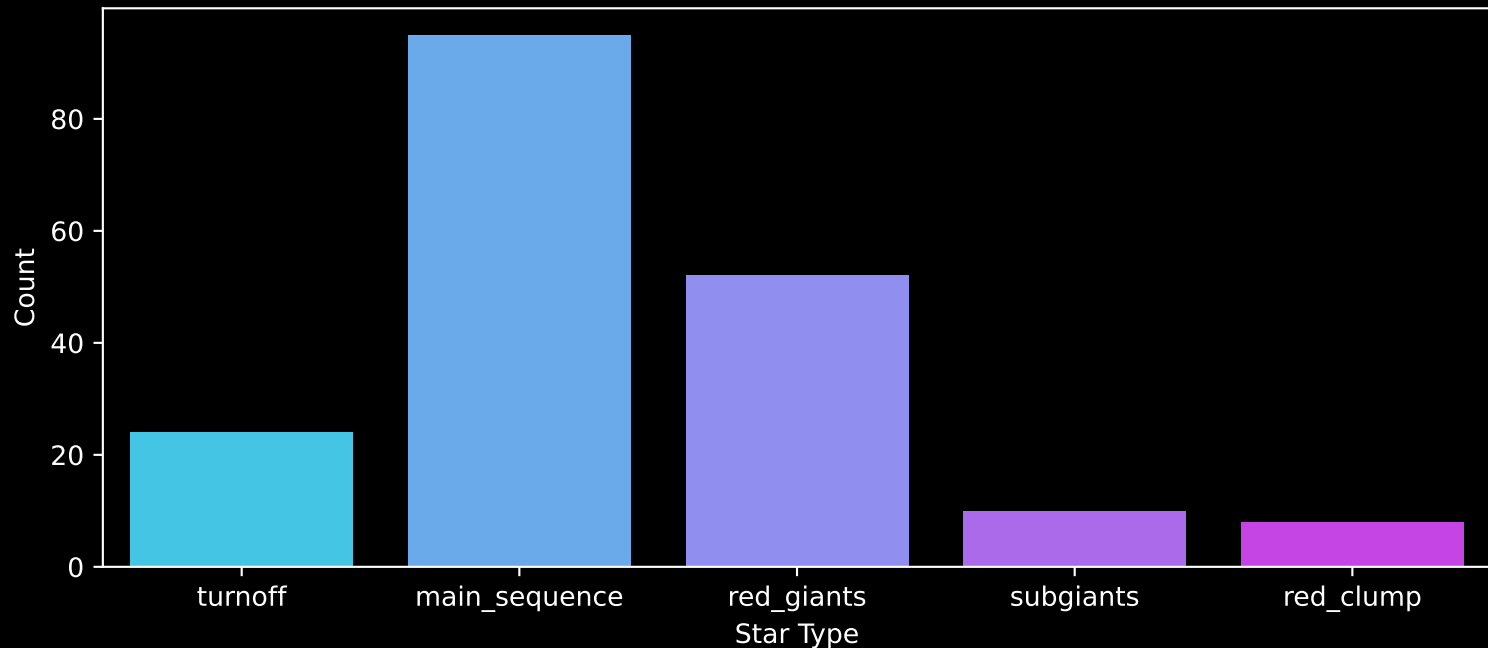
APOGEE DR17 Field: [K2_C6_321+50_btx] Count plot of Star Type
