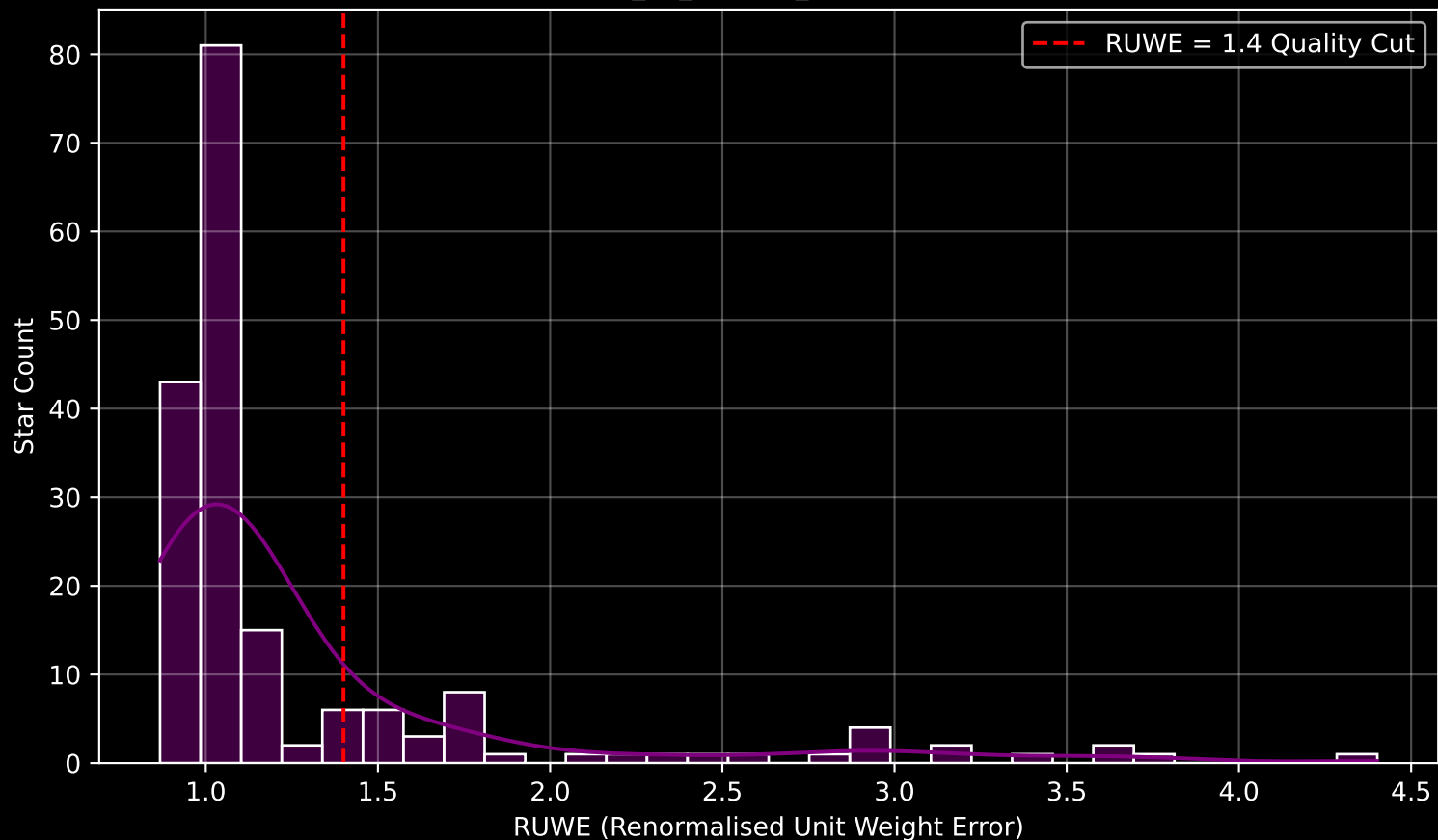
GAPOGEE DR17 Field [K2_C6_321+50_btx] RUWE Distribution (n= 182)
